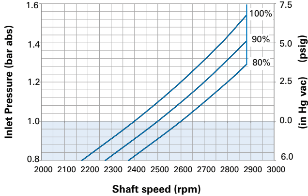
Inlet pressure vs. Speed @ 49°C (120°F)
