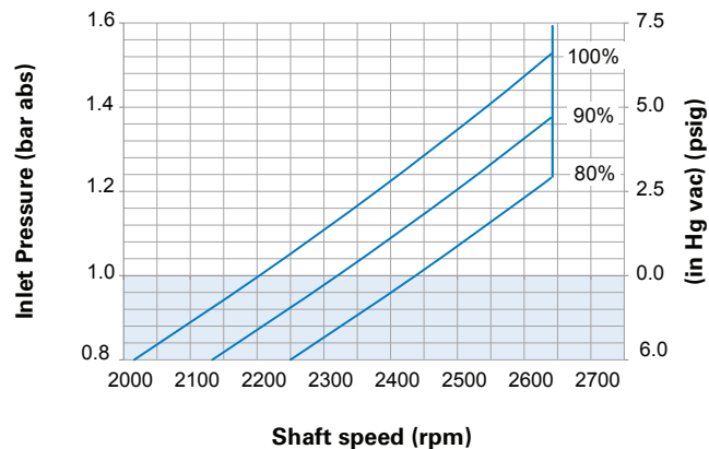
Inlet pressure versus speed @ 49°C (120°F)
