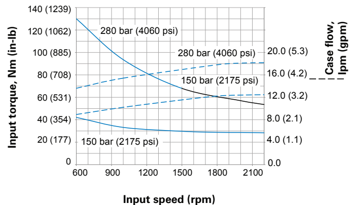
Input torque and case flow cut-off @ 49°C (120°F)
