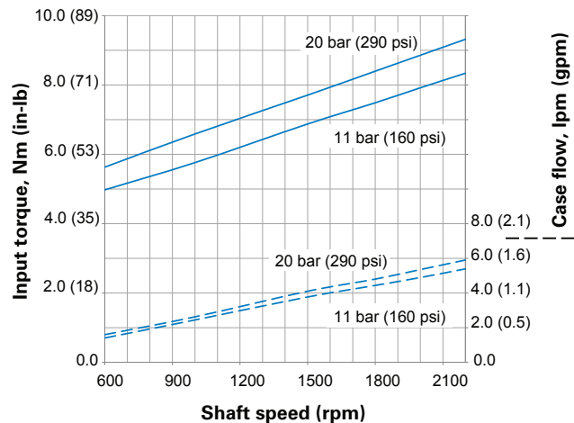
Input torque and case flow stand-by @ 49°C (120°F)
